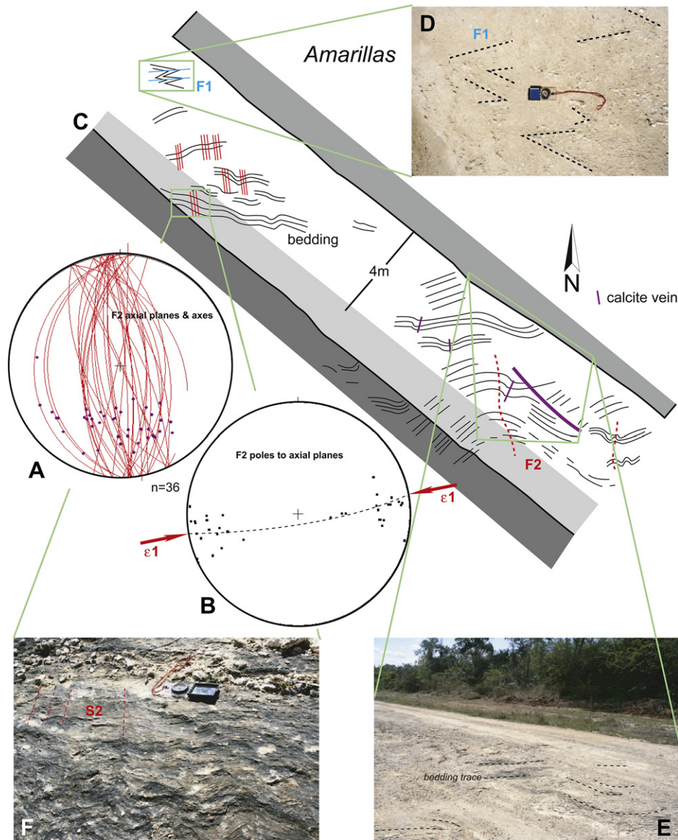
Fig. 6. Form trace map of the small road floor exposure of the Las Amarillas block (Placetas belt; see Fig. 2 for location). The deformation of the Las Amarillas block is characterized by a second phase of open folding and locally associated axial plane cleavage, which overprints a first phase of isoclinal folding. The spread in poles to F2 axial planes and F2 fold axes may indicate a third, weaker phase of folding, the shape of which cannot be constrained in this outcrop. (E) The typical outcrop used for study of the structure.
